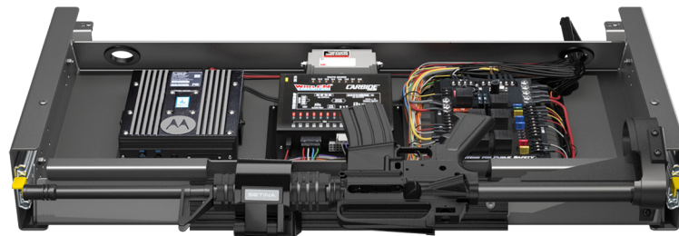
PASSENGER CAR TRUNK TRAY ( Electronics Not Included )
